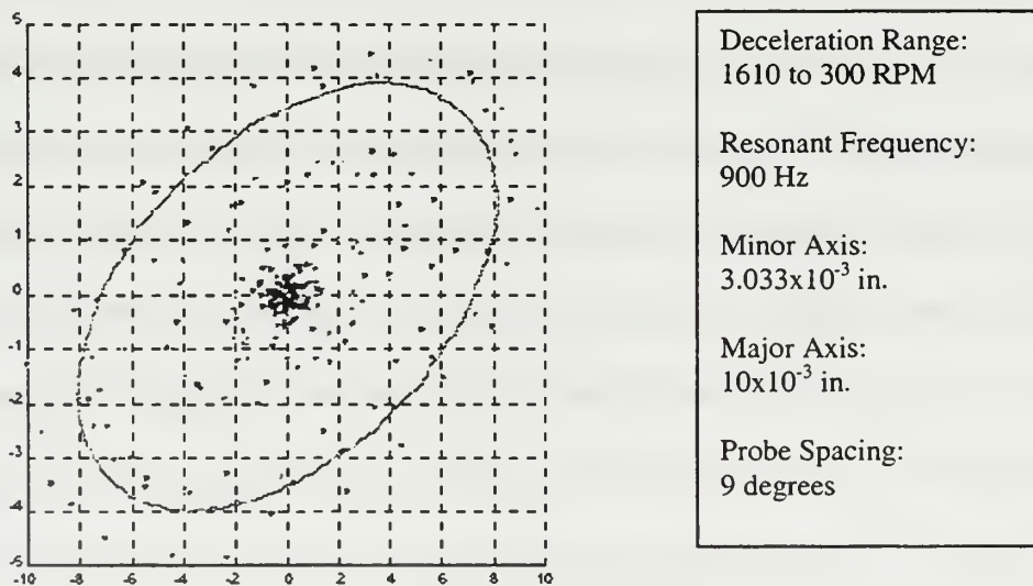
Figure 4.7 Analysis of Test Data (0.001 in. per division)
